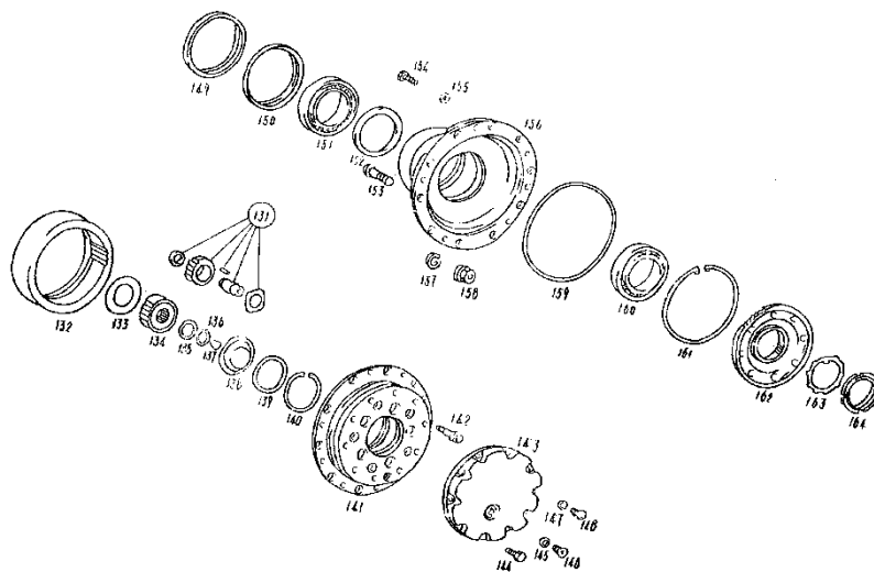
驱动前桥总成Front axle assembly
