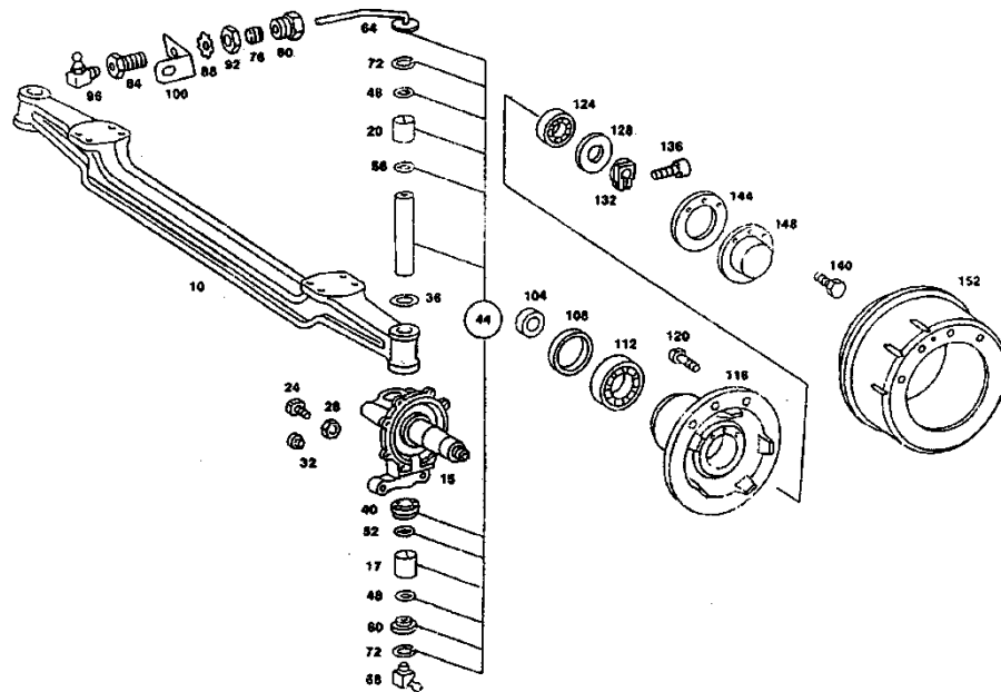
非驱动前桥总成Front axle assembly
